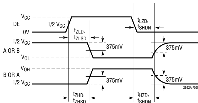
Figure 5. Driver Enable and Disable Timing Measurements
