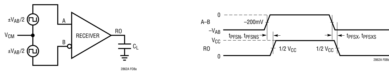
Figure 8. Failsafe Delay Measurements
