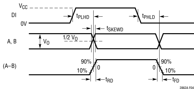
Figure 4. Driver Timing Measurement
