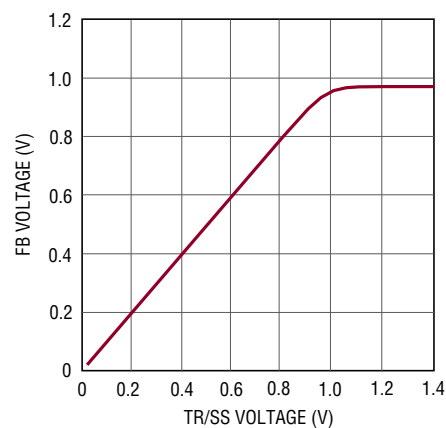
Soft-Start Tracking
