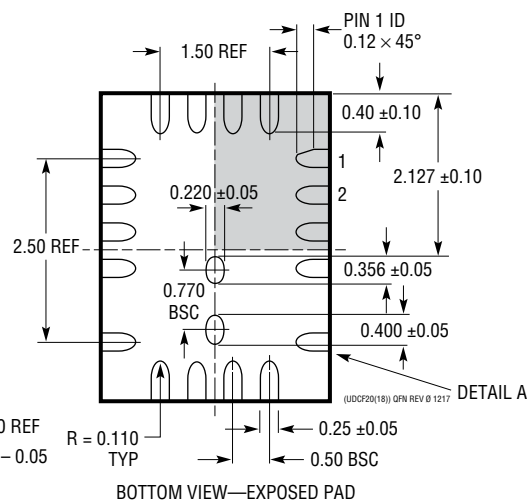
BOTTOM VIEW—EXPOSED PAD
