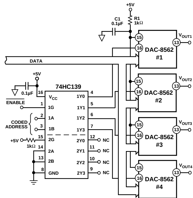
Figure 40. Decoding Multiple DAC8562s Using the \overline{\text{CE}} Pin
