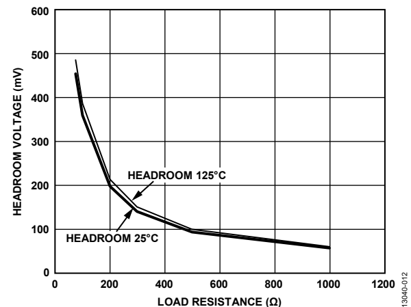
Figure 12. Typical Headroom Voltage vs. Load Resistance for VDACC4, AV_{DD} = 3\text{ V} ; Headroom = AV_{DD} - \text{VDAC Output Voltage}
