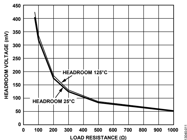
Figure 11. Typical Headroom Voltage vs. Load Resistance for VDACC0, AV_{DD} = 3\text{ V} ; Headroom = AV_{DD} - \text{VDAC Output Voltage}
