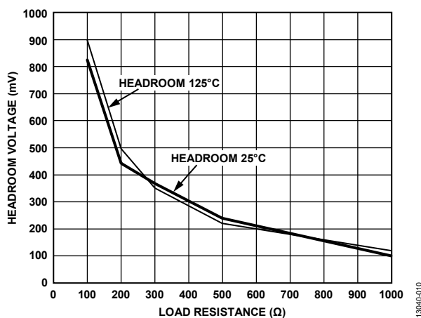
Figure 10. Typical Headroom Voltage vs. Load Resistance for VDACC2, AV_{NEG} = -5\text{ V} ; Headroom = AV_{NEG} - \text{VDAC Output Voltage}
