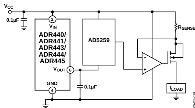
Figure 40. Programmable Current Source
