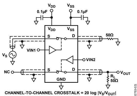
Figure 21. Channel-to-Channel Crosstalk
