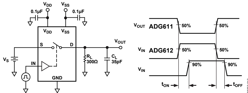
Figure 17. Switching Times
