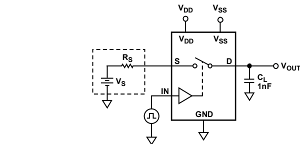
Figure 19. Charge Injection
