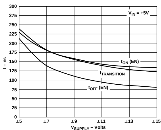
Figure 9. Switching Time vs. Bipolar Supply
