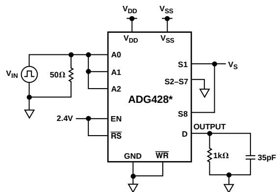
Test Circuit 6. Break-Before-Make Delay, t_{\text{OPEN}}
