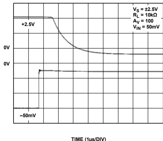
Figure 40. Positive Overload Recovery
