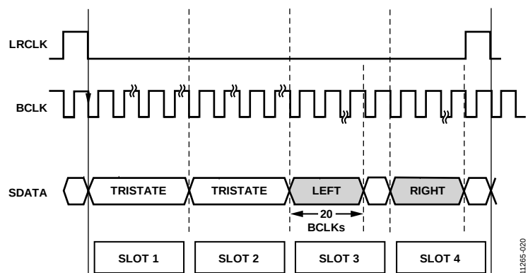
Figure 20. TDM4 Channel 3 and Channel 4, CONFIG Pin Open
