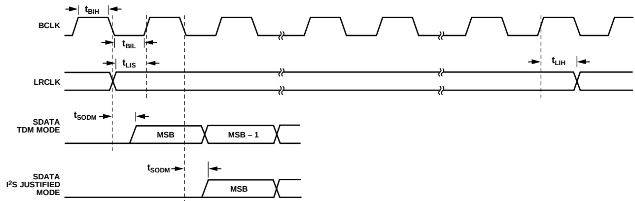
Figure 13. Serial Port Timing Diagram
